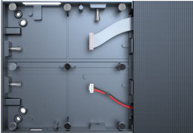
▲ Internal bolts and cables
